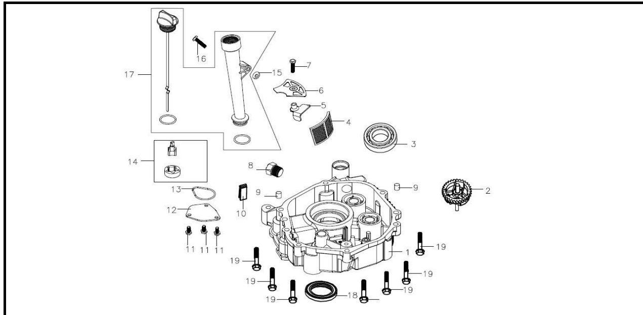
曲轴箱盖 (Crankcase Cover)
