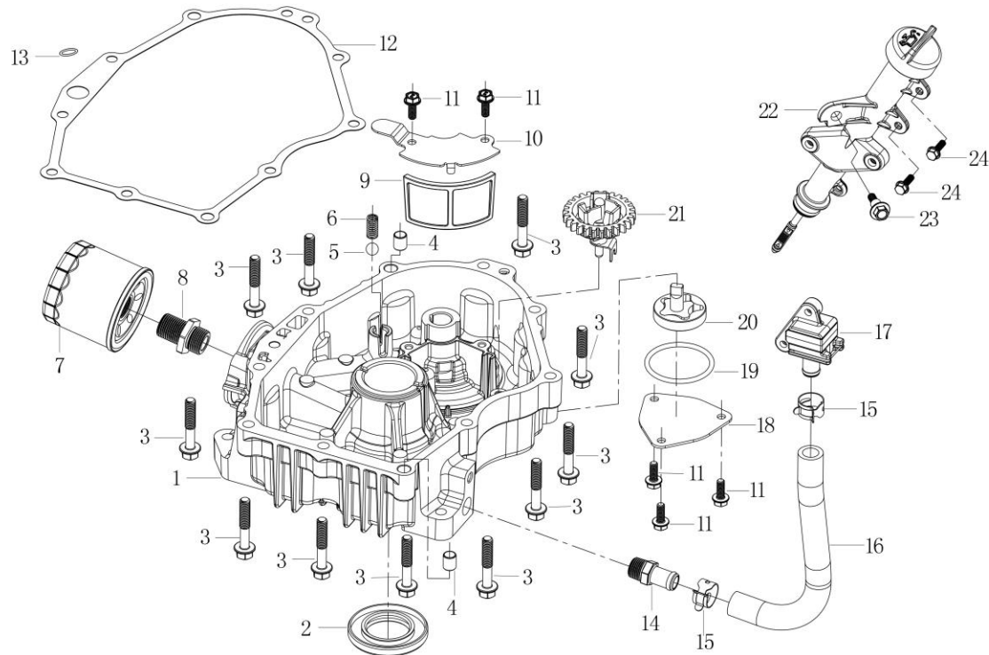
曲轴箱盖 (CRANKCASE COVER)
